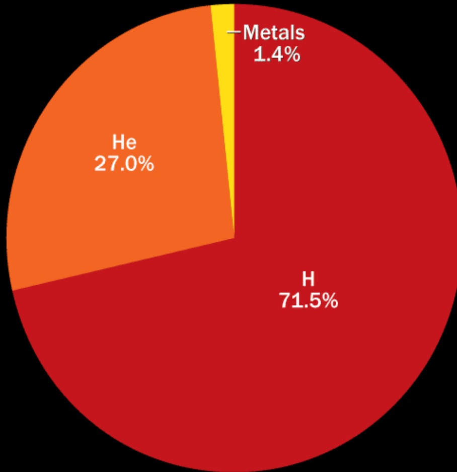
Total solar composition
